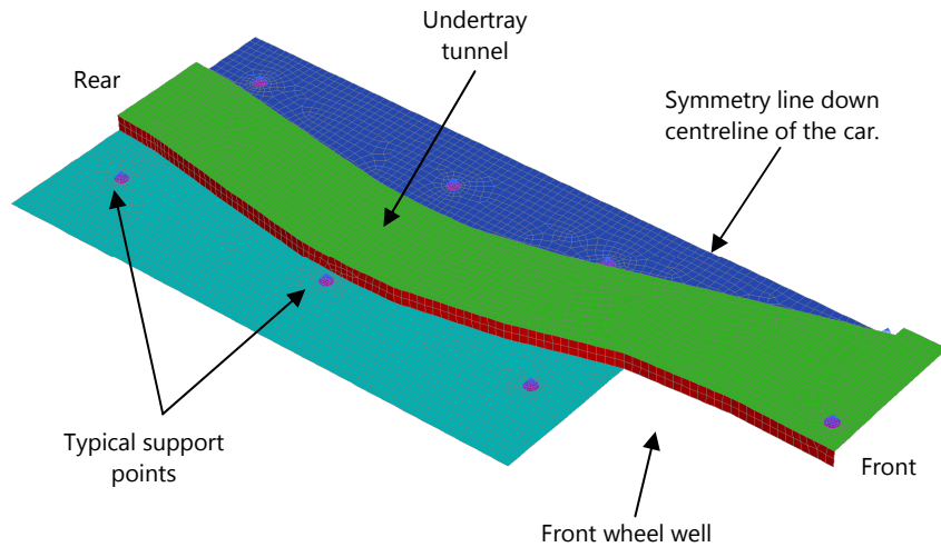
FEA model of the carbon fibre undertray.
