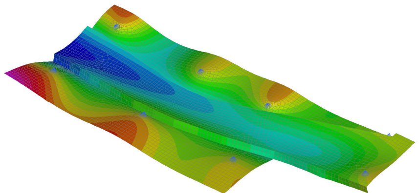
Vertical deflection results for combined pattern wind load and dead loading
