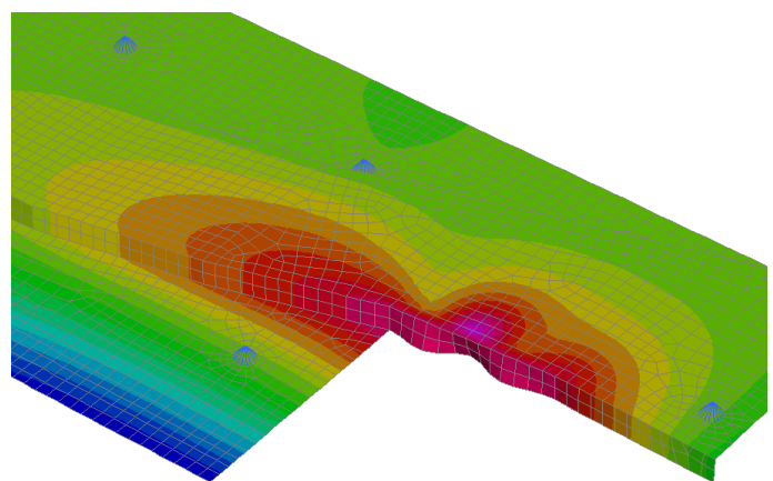
Linear buckling analysis results showing distortion buckling of the forward tunnel face.
