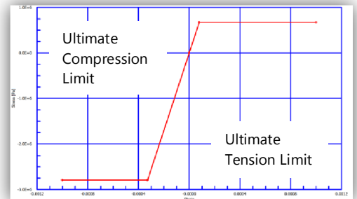
Tri-Linear Stress Strain Curve for the AAC Material
