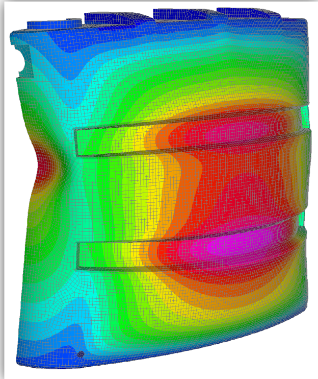
Buckled shape of the 2,000 litre slimline tank.
