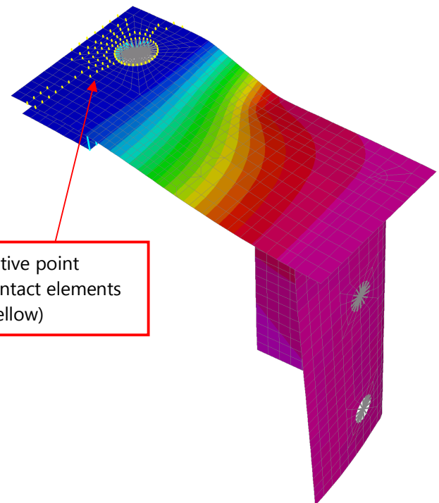
Displaced Shape of the footplate assembly under vertical loads with active point contact elements shown in yellow.
