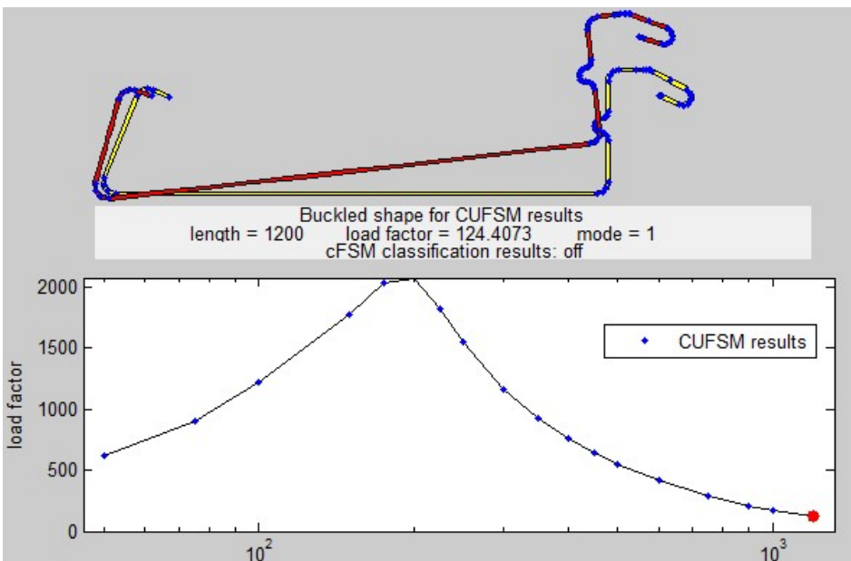
CUFSM analysis of stainless steel rail
