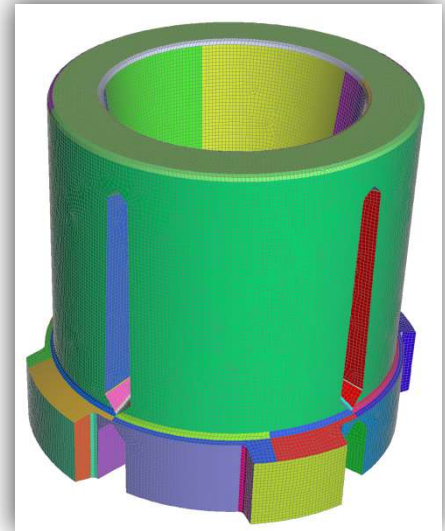
FEA Model of the 5,000 litre underground septic tank
