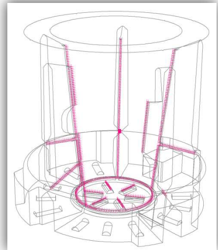
Outline wire frame of FEA Model indicating kiss-off zones with rigid link elements (red)
